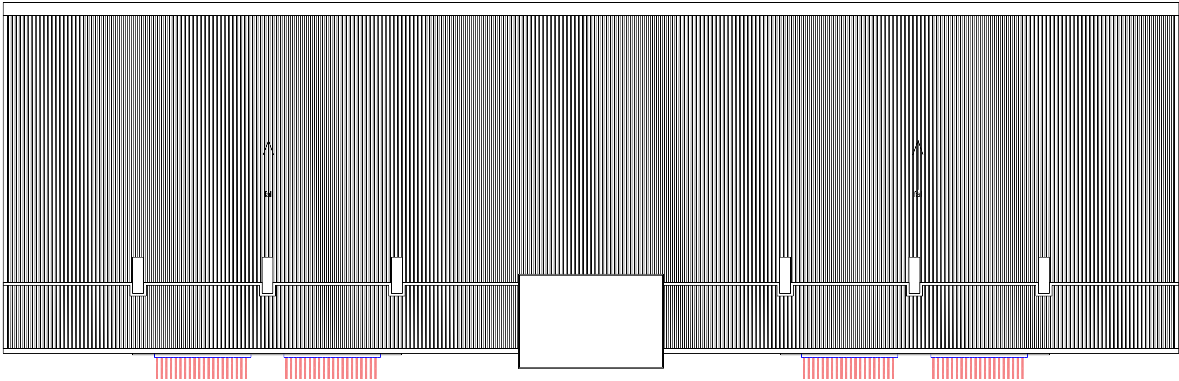
ROOF PLAN - ARCADE BUILDING scale 1:100
