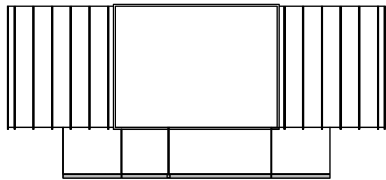
ROOF PLAN - STATION BUILDING scale 1:100
