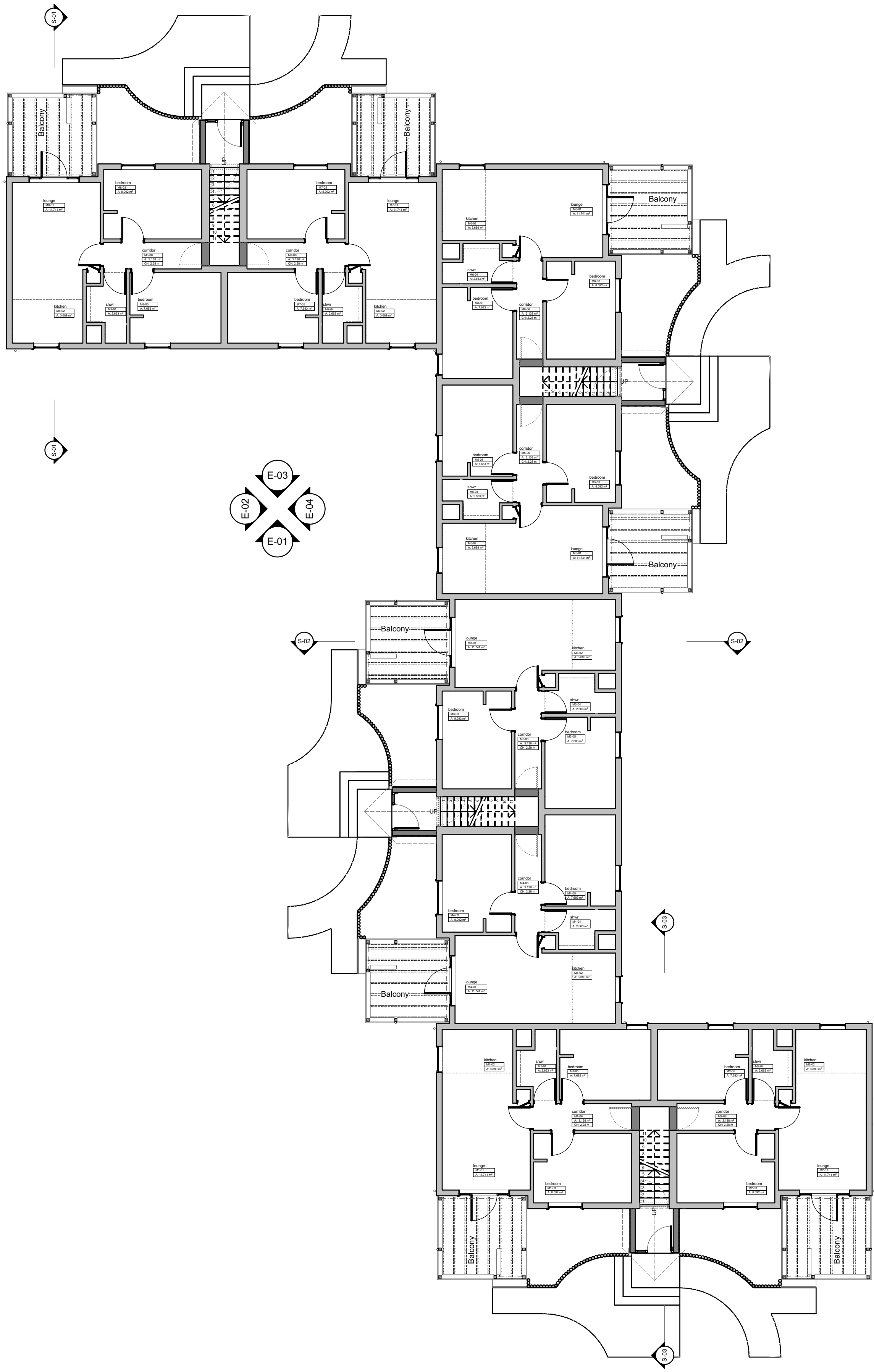
A1 Ground Floor 1:100
